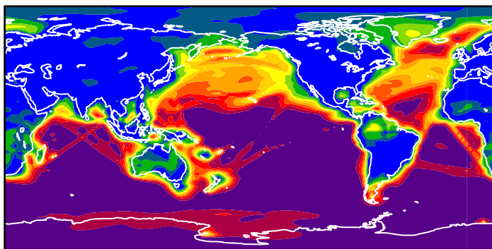
(c) Percentage of total SO 2 from DMS
