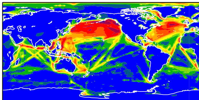
(e) Percentage of total sulfate from shipping
