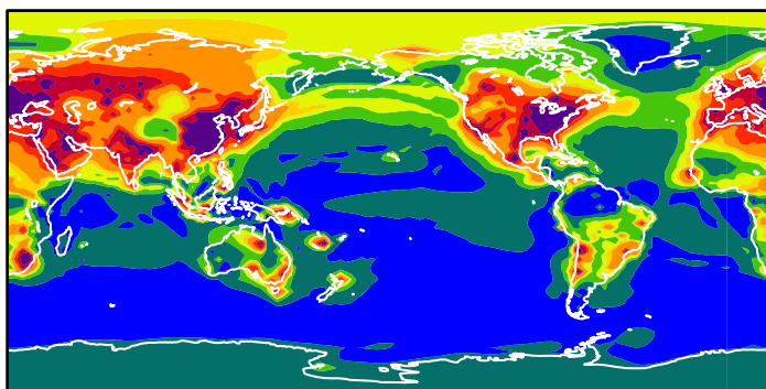
(a) Total SO 2
