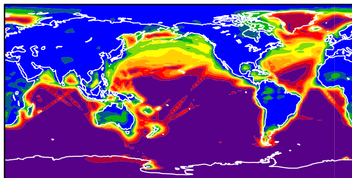
(f) Percentage of total sulfate from DMS
