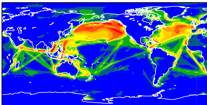
(b) Percentage of total SO 2 from shipping
