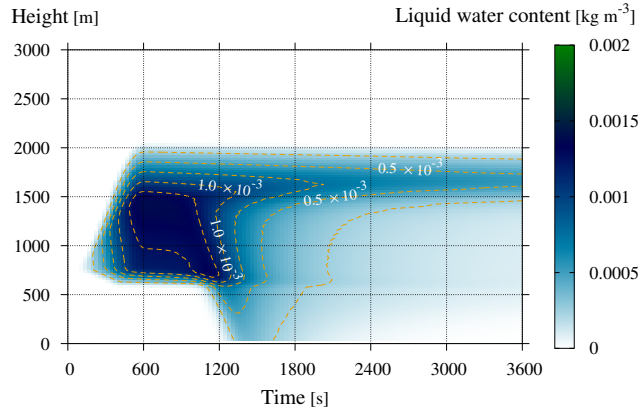
(b) MSSG-Bin
