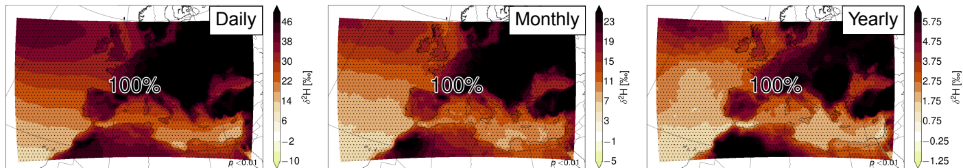
(a) \delta^2\text{H}_{fin}
