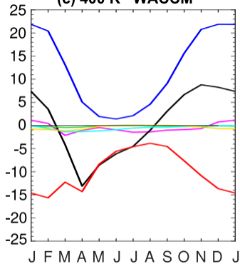
(c) 400 K WACCM
