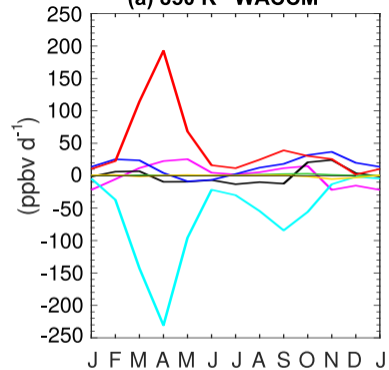
(a) 850 K WACCM
