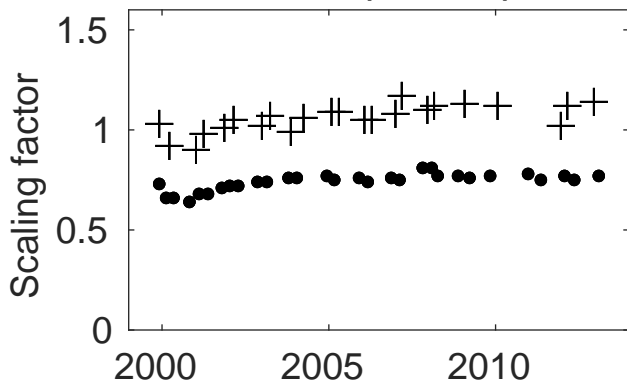
Channel 5 (380 nm)
