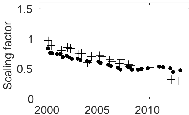
Channel 3 (320 nm)
