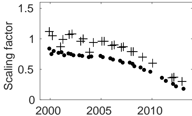
Channel 2 (312 nm)
