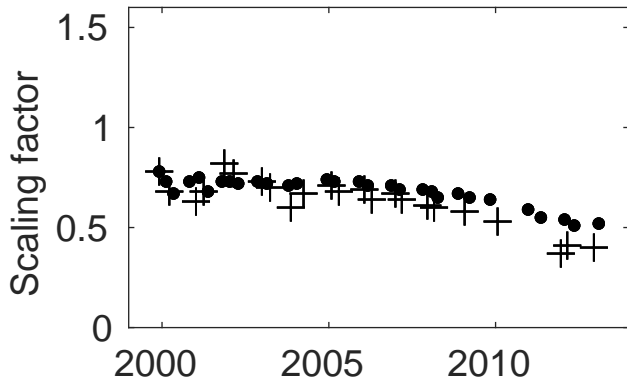
Channel 1 (305 nm)
