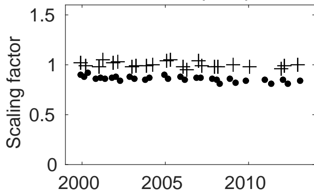
Channel 6 (PAR)
