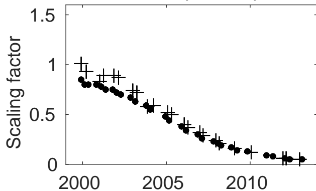
Channel 4 (340 nm)
