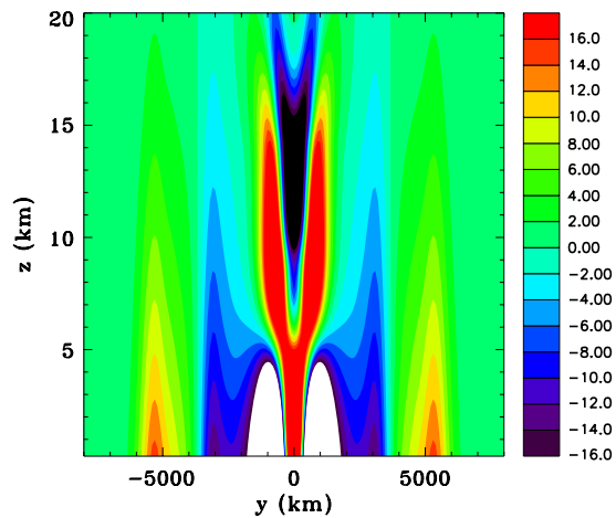
(c) Total energy perturbation
