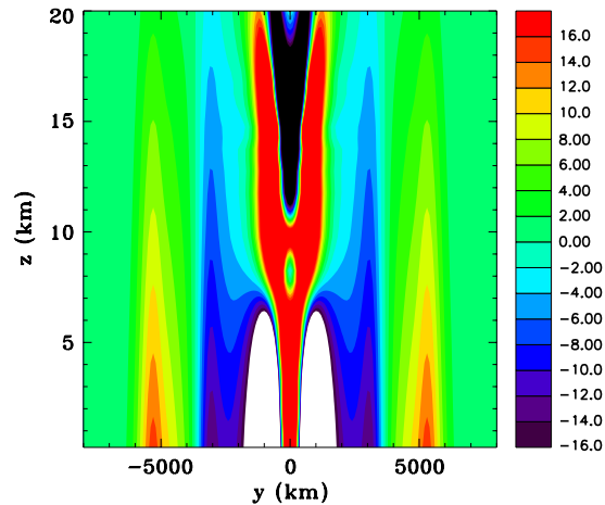
(c) Total energy perturbation
