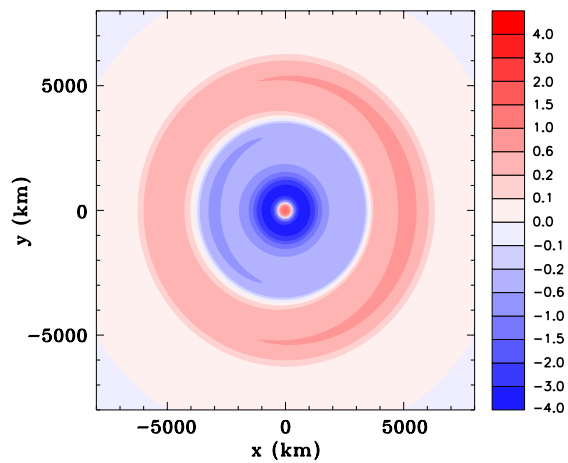
(e) Vertically summed mass change
