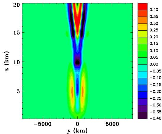
(a) Potential temperature perturbation
