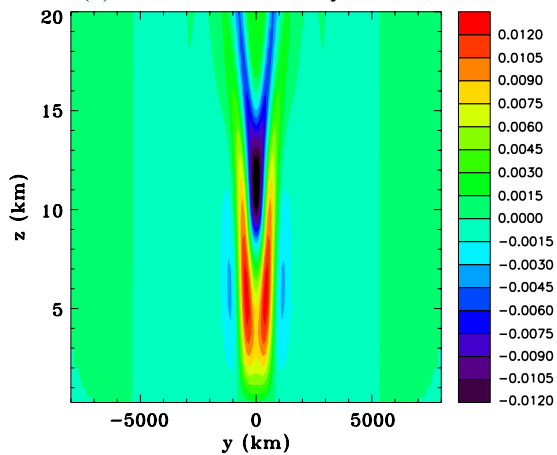
(b) Vertical velocity
