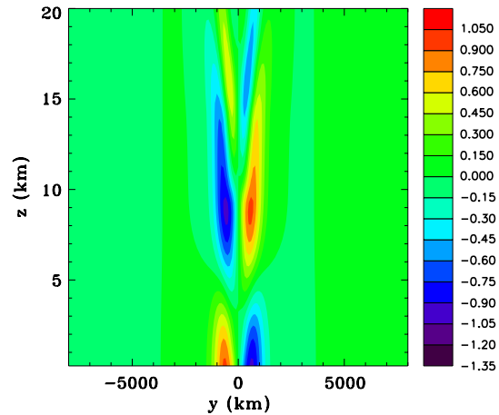
(c) y component of velocity ( v )
