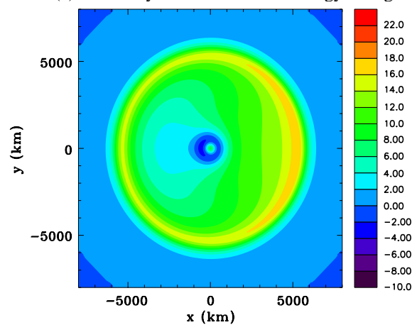
(c) Vertically summed internal energy change
