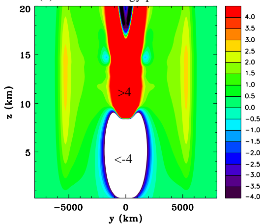
(b) Potential energy perturbation
