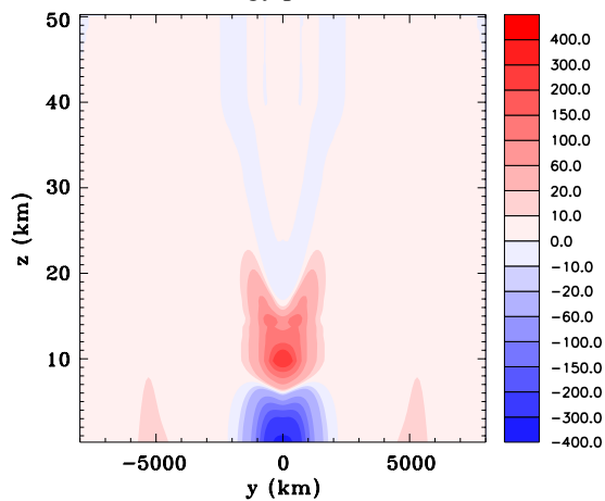
(e) Total energy perturbation
