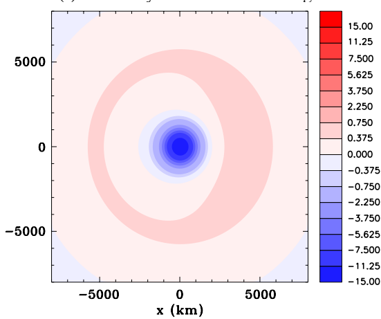
(f) Vertically summed mass change
