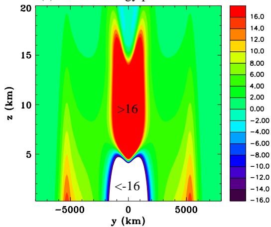
(a) Internal energy perturbation
