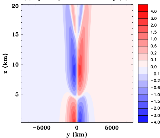
(e) y component of velocity ( v )
