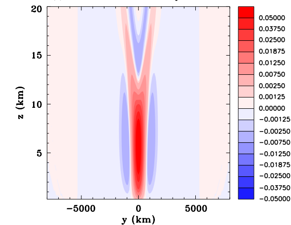
(f) Vertical velocity
