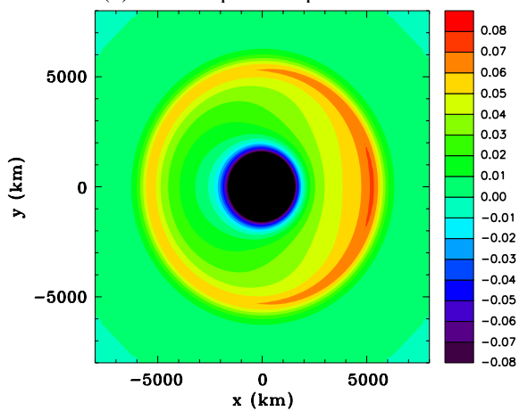
(b) Surface pressure perturbation
