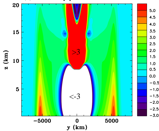
(c) Density perturbation
