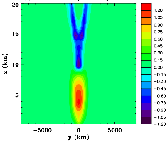
(a) Potential temperature perturbation
