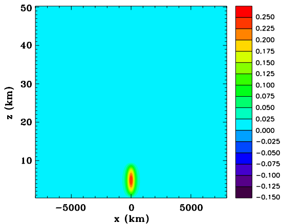
(a) Heating rate
