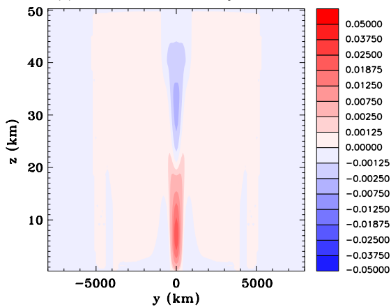
(e) Vertical velocity
