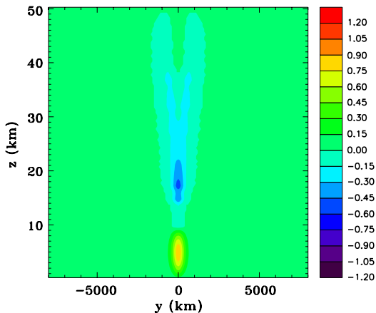
(b) Potential temperature perturbation
