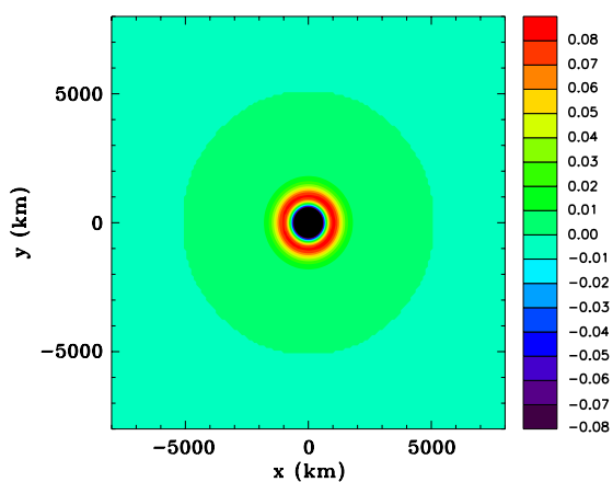
(f) Surface pressure perturbation
