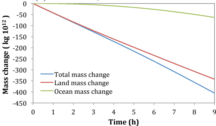
(b) Mass changes over land and ocean
