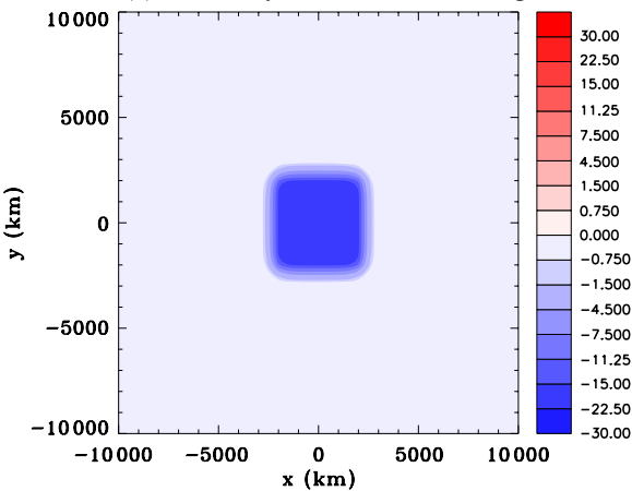
(e) Vertically summed mass change
