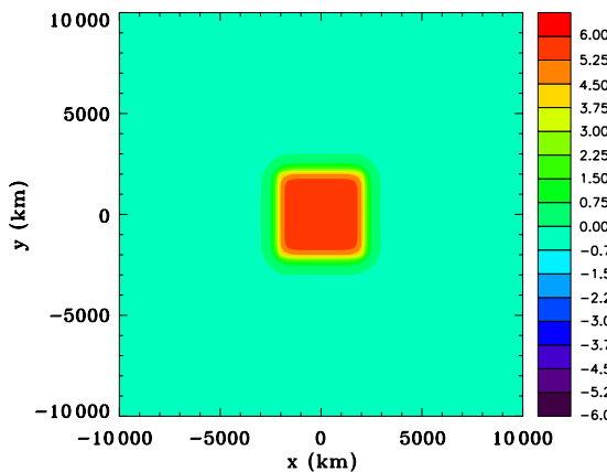
(a) Potential temperature perturbation
