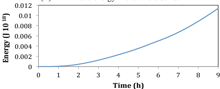
(c) Total energies over land and ocean
