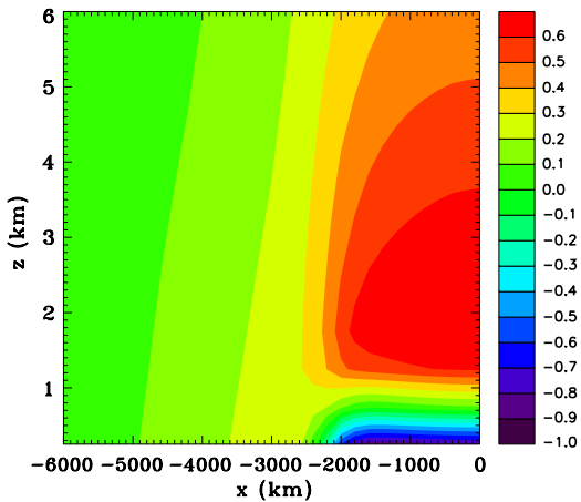
(a) Pressure perturbation
