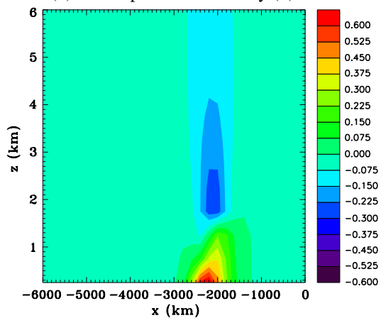
(b) x-component of velocity ( u )
