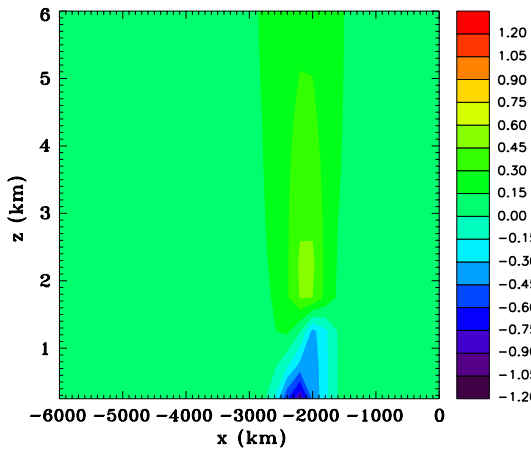
(c) y-component of velocity ( v )
