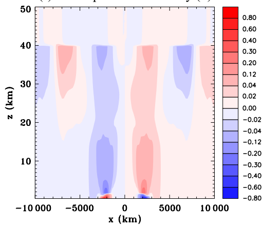
(f) x component of velocity (u)
