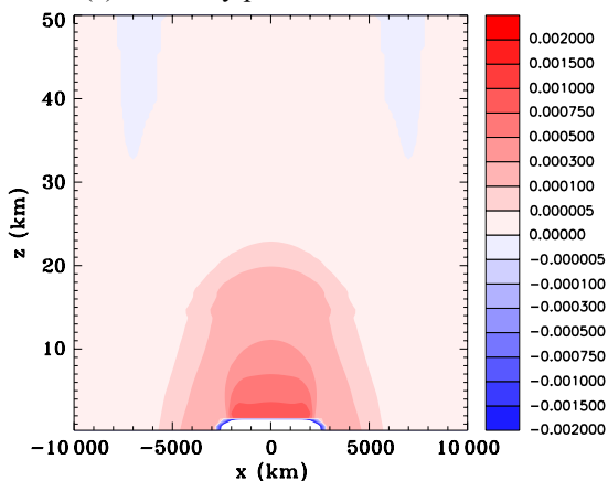
(c) Density perturbation
