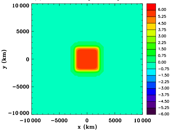
(a) Potential temperature perturbation
