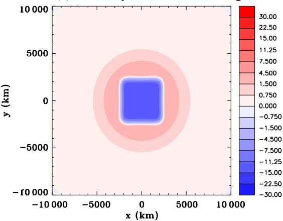
(e) Vertically summed mass change
