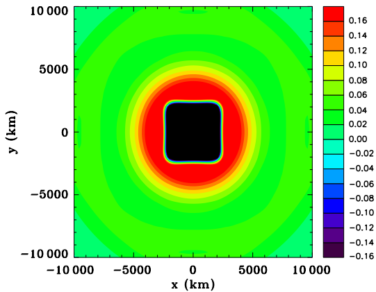
(b) Pressure perturbation
