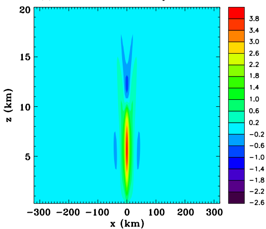
(e) Vertical velocity
