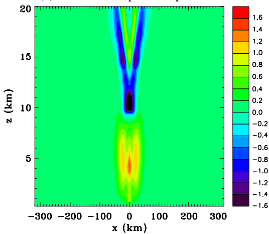
(a) Potential temperature perturbation
