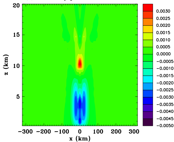
(c) Density perturbation
