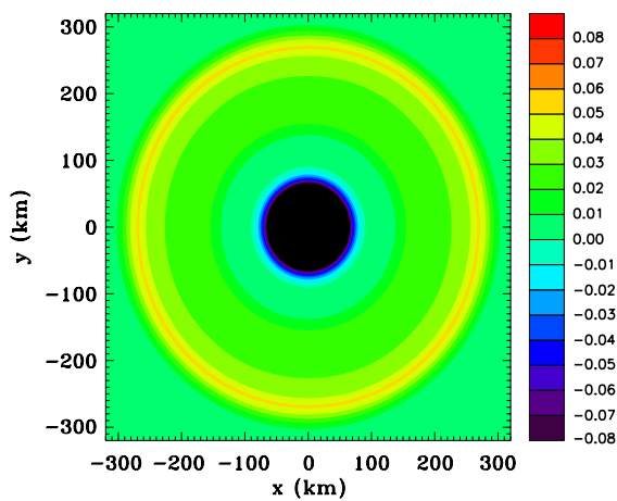
(f) Surface pressure perturbation
