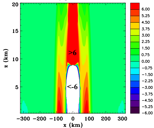
(a) Density perturbation t=5 m
