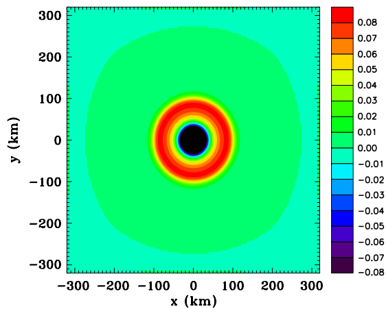
(b) Surface pressure perturbation t=5 m
