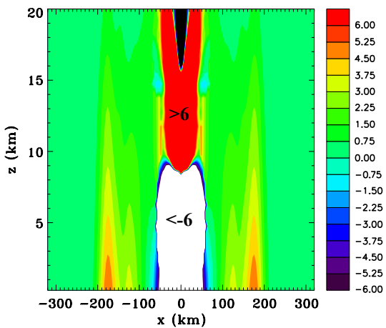
(c) Density perturbation t=10 m
