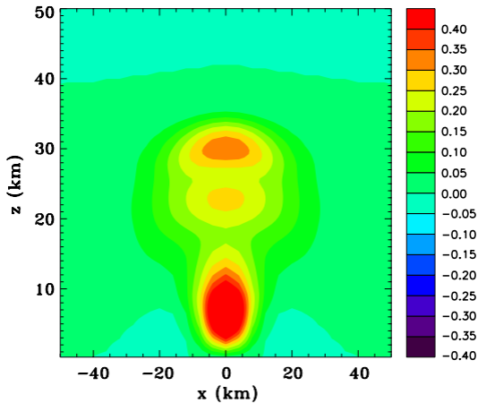
(b) Vertical velocity, t=90 s
