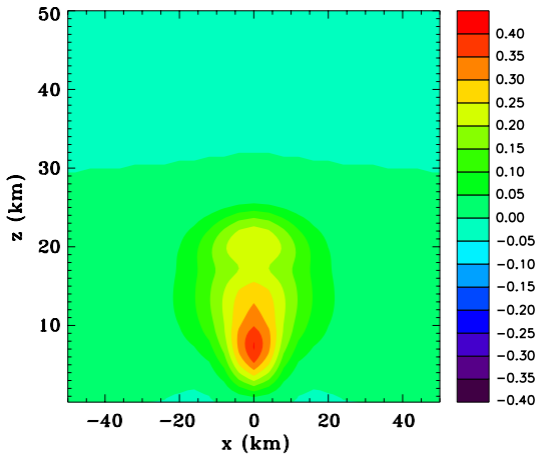
(a) Vertical velocity, t=60 s
