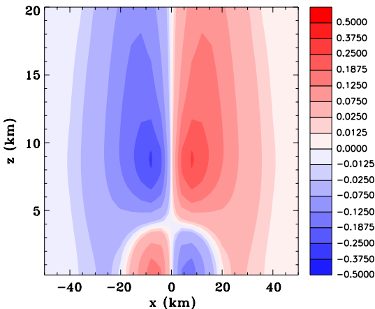
(a) x component of velocity ( u ), t = 80 s
