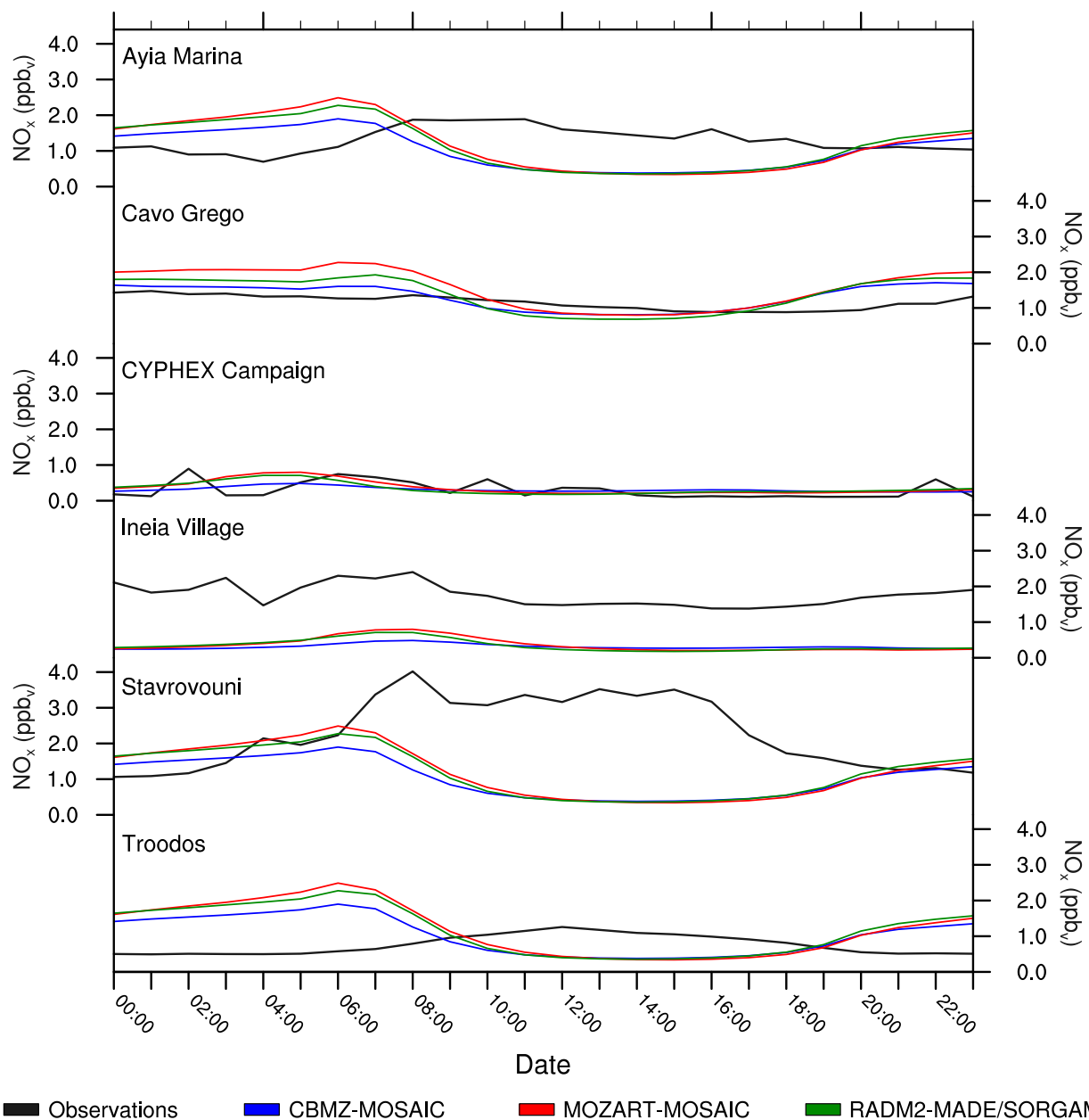
Figure S3. Observed (grey line) and modelled \text{NO}_x monthly mean diurnal cycles from the CBMZ-MOSAIC (blue line), MOZART-MOSAIC (red line), and RADM2-MADE/SORGAM (green line) mechanisms.
