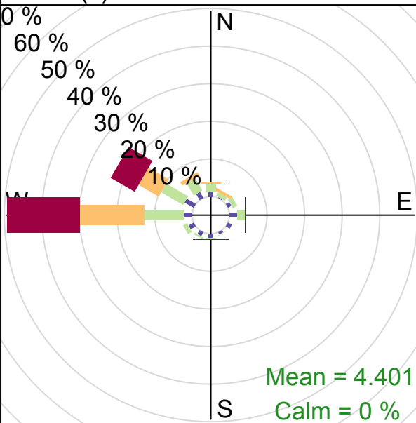
(c) MOZART-MOSAIC
