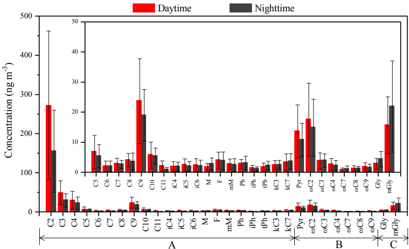
A: Dicarboxylic acids; B: Ketocarboxylic acids; C: \alpha -dicarbonyls
