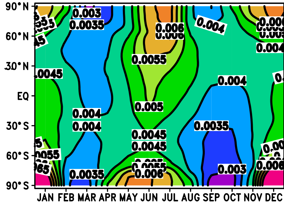
(c) WACCM Ca/Na
