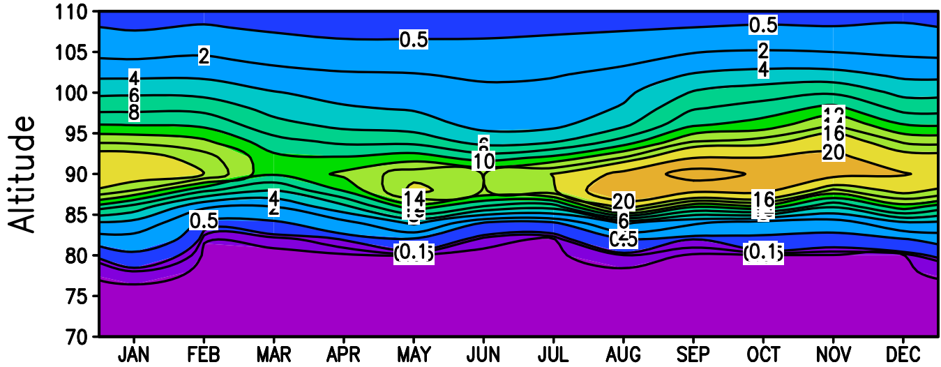
(b) Standard WACCM-Ca ( \text{cm}^{-3} )
