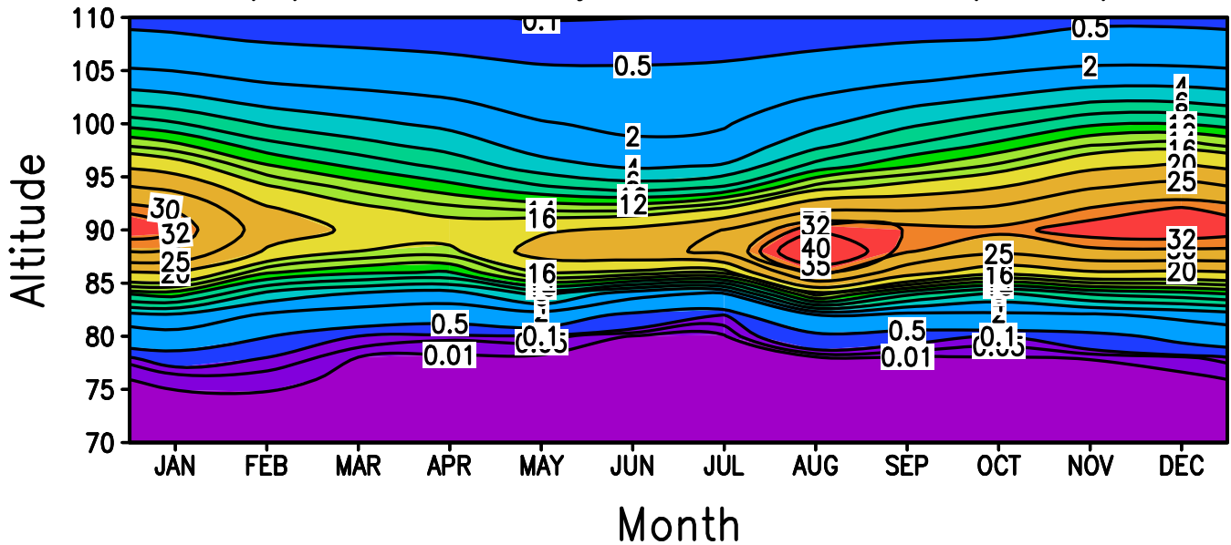
(c) Sensitivity WACCM-Ca ( \text{cm}^{-3} )
