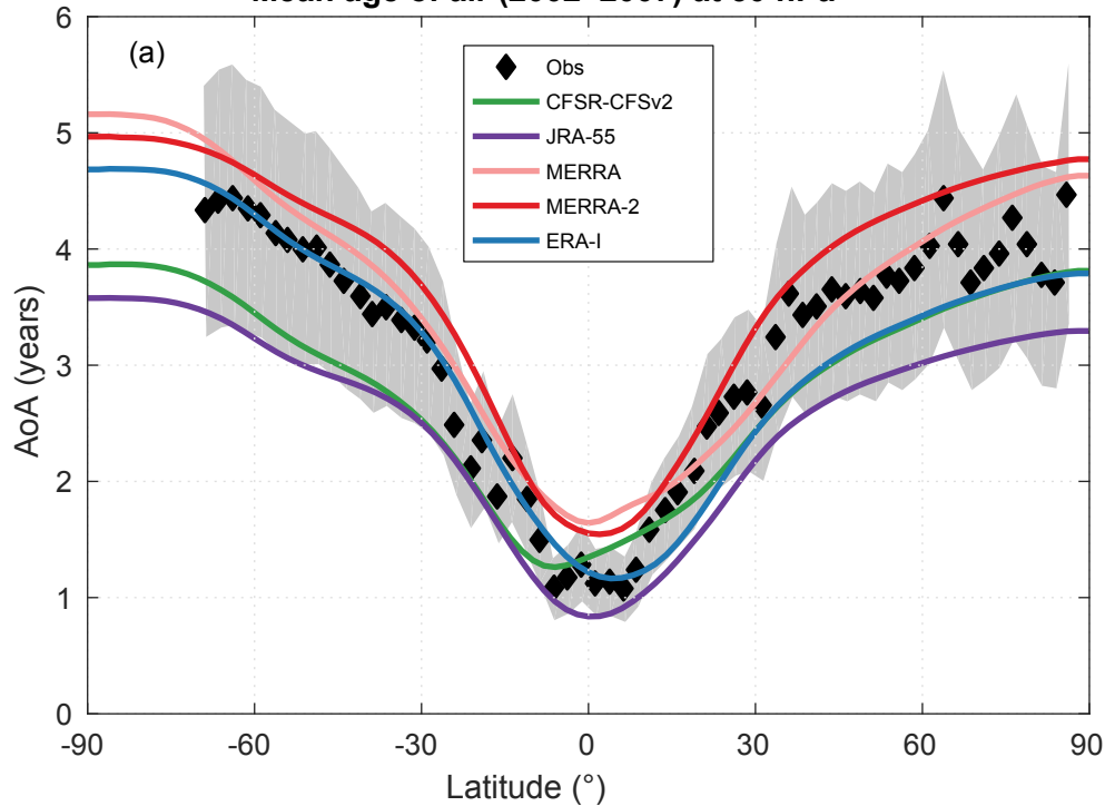
Mean age of air (2002–2007) at 50 hPa
