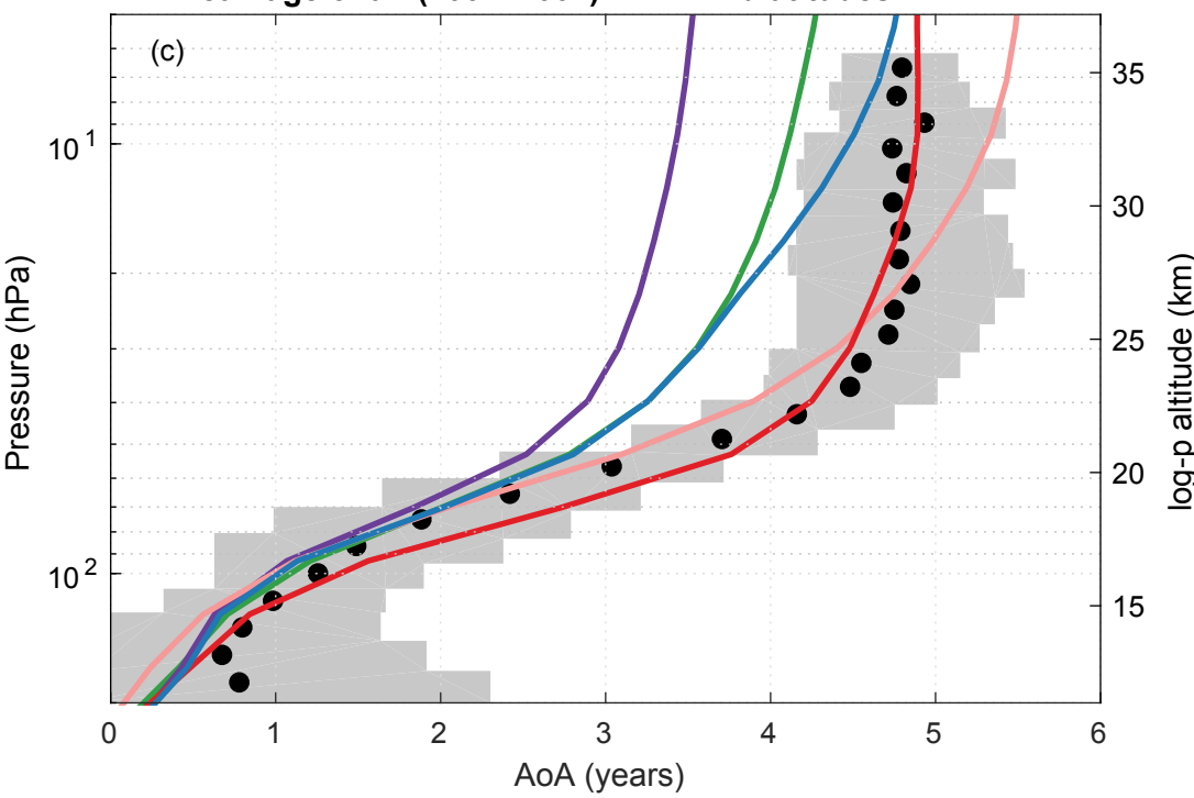
Mean age of air (2002–2007) in NH midlatitudes
