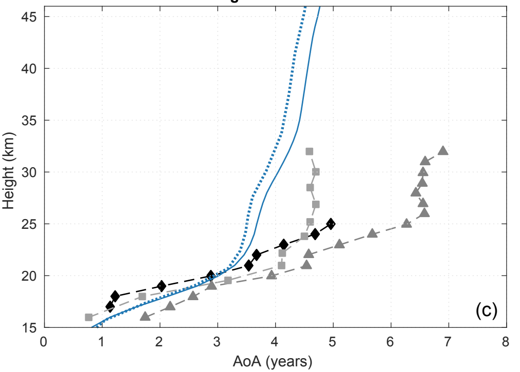
Mean age of air at 40° N
