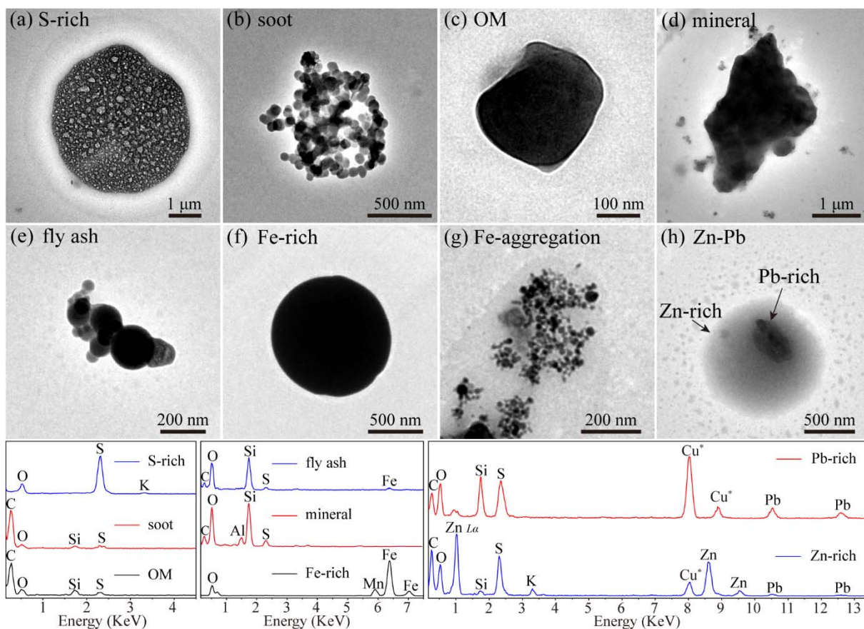
Figure S2. Typical TEM images and EDS spectra of different basic types of individual particles. (a) S-rich, (b) soot, (c) organic matter (OM), (d) mineral, (e) fly ash, and (f-h) metal particles including Fe-rich, Fe-aggregation, and Zn-Pb.
