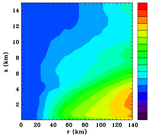
(a) Angular momentum t = 48 h
