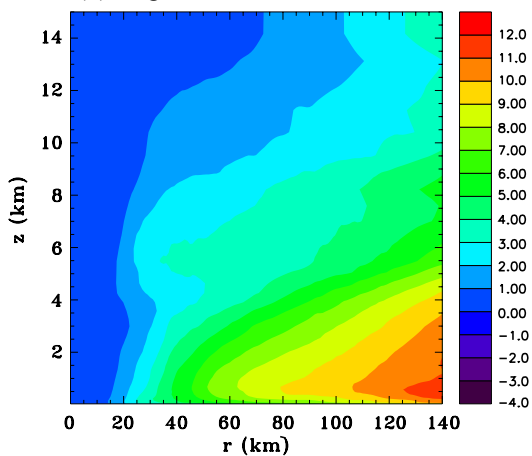
(b) Angular momentum t = 60 h
