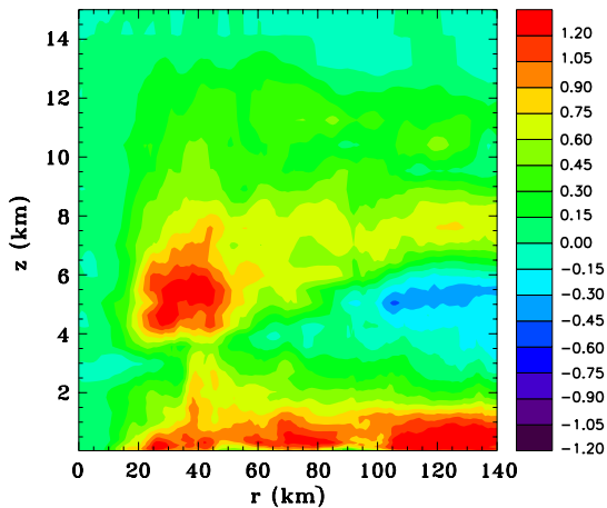
(c) Angular momentum change
