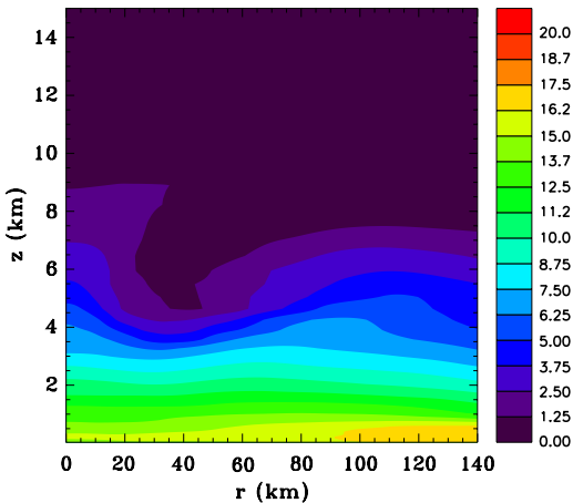
(b) Vapour mixing ratio 12 h
