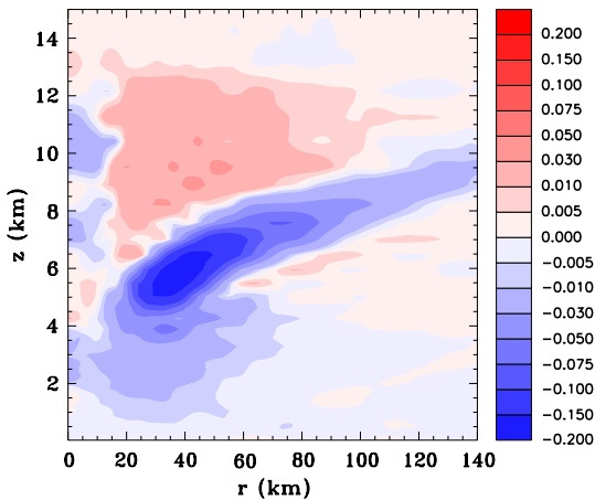
(a) Time-averaged vertical velocity
