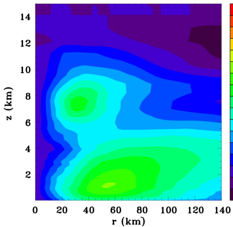
(c) Tangential velocity
