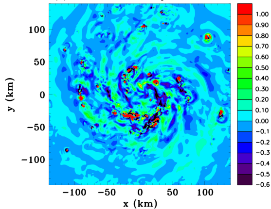
(c) Vertical velocity z = 4.6 km 48 h
