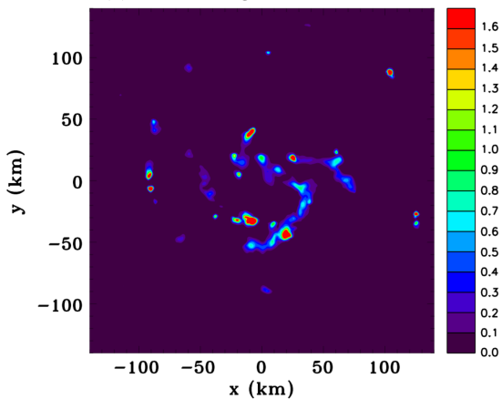
(a) Ice mixing ratio z = 5.5 km 48 h
