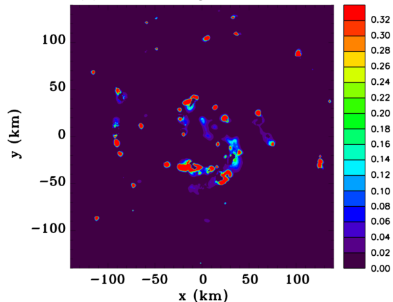
(b) Rain mixing ratio z = 3.9 km 48 h
