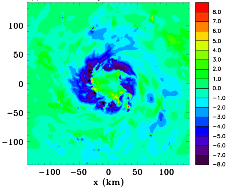
(a) Radial velocity z = 6.5 \text{ km} 60 h
