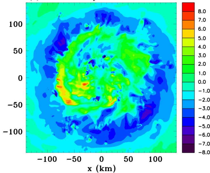
(b) Radial velocity z = 8.9 \text{ km} 60 h
