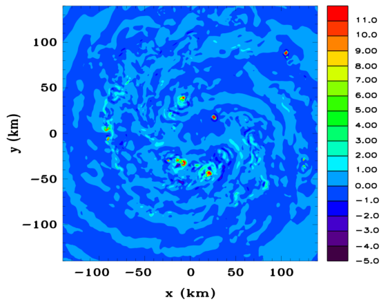
(a) Vertical velocity z = 9.5 km 48 h
