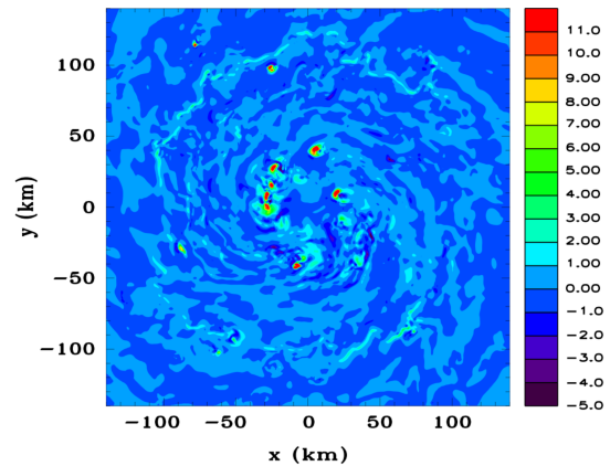
(c) Vertical velocity z = 9.5 km 60 h
