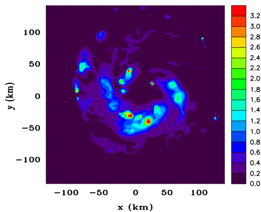
(b) Hydrometeors z = 9.5 km 48 h
