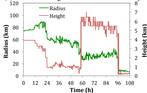
(c) Radius and height of the maximum velocity
