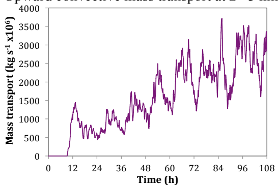
(f) Upward convective mass transport at z= 3 km
