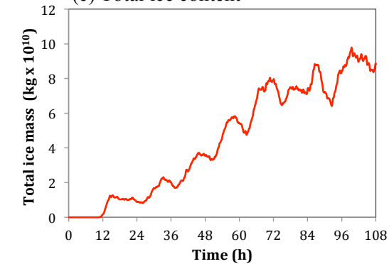
(e) Total ice content
