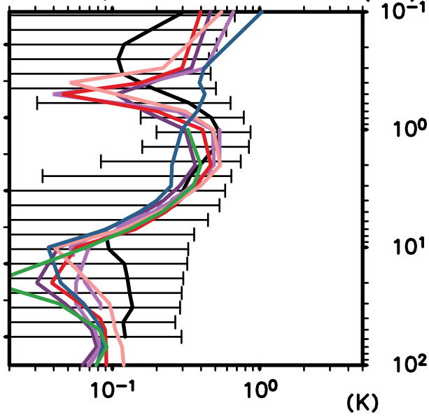
(c) Amplitude (30–45° N) (hPa)
