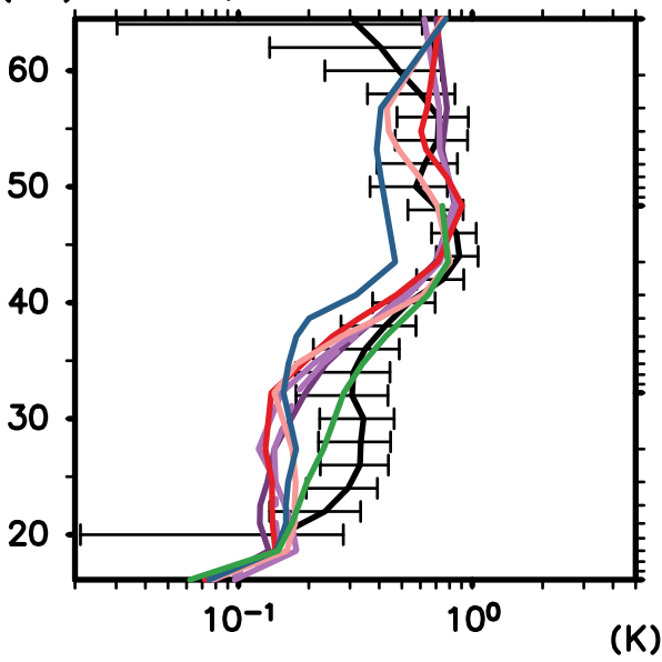
(a) Amplitude (15° S–15° N)
