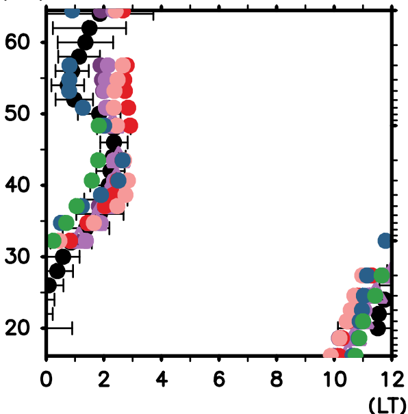
(b) Phase (15° S–15° N)
