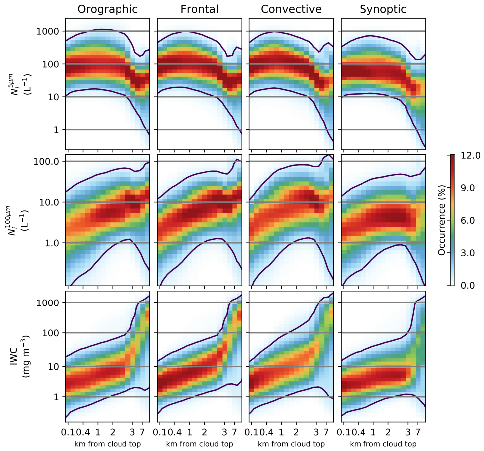
Figure S1: As Fig. 5 in the main paper, but for clouds with tops between -60 and 0 . Showing the retrieved properties as a function of the distance from the cloud top. Note the non-linear scale on the horizontal axis
