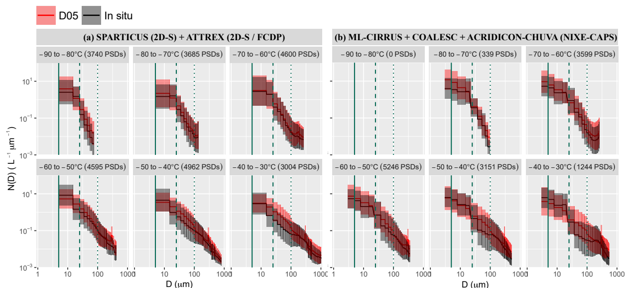
Figure 1. (a) Mean PSDs measured (black lines) during SPARTICUS and ATTREX, averaged per 10^\circ\text{C} temperature bin (from -90 to -30^\circ\text{C} ). Black contours indicate one standard deviation around the mean. The mean and spread of one-to-one predictions by the D05 parameterization are similarly indicated in red. The total number of PSDs in each T_c bin is indicated in the panel heading and the relative contributions from each campaign can be deduced from Fig. S1. Vertical plain, dashed and dotted green lines indicate D = 5, 25 and 100 \mu\text{m} , respectively. The SPARTICUS data with T_c < -60^\circ\text{C} are ignored here to avoid contaminating FCDP measurements with uncertainties arising from the first size bins of 2D-S. (b) Similar to (a) but for the ML-CIRRUS, COALESC and ACRIDICON-CHUVA campaigns.
