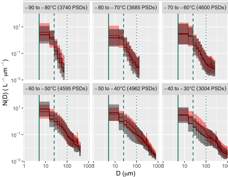
(a) SPARTICUS (2D-S) + ATTREX (2D-S / FCDP)
