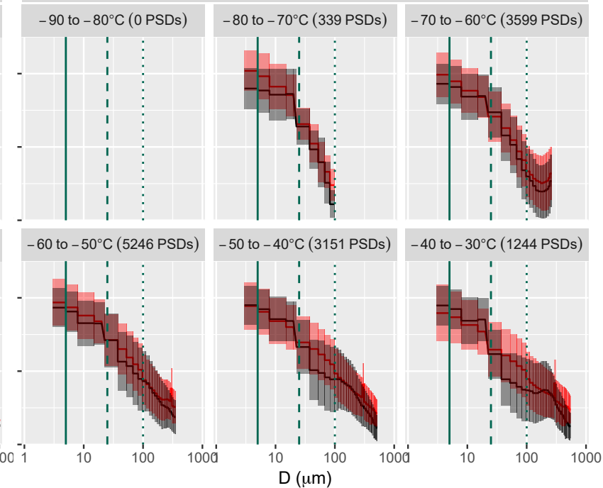
(b) ML-CIRRUS + COALESC + ACRIDICON-CHUVA (NIXE-CAPS)
