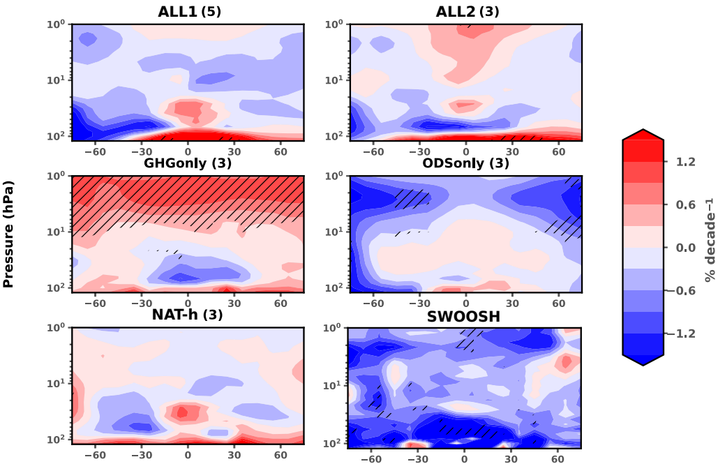
(a) Linear trends, 1984-2016*
