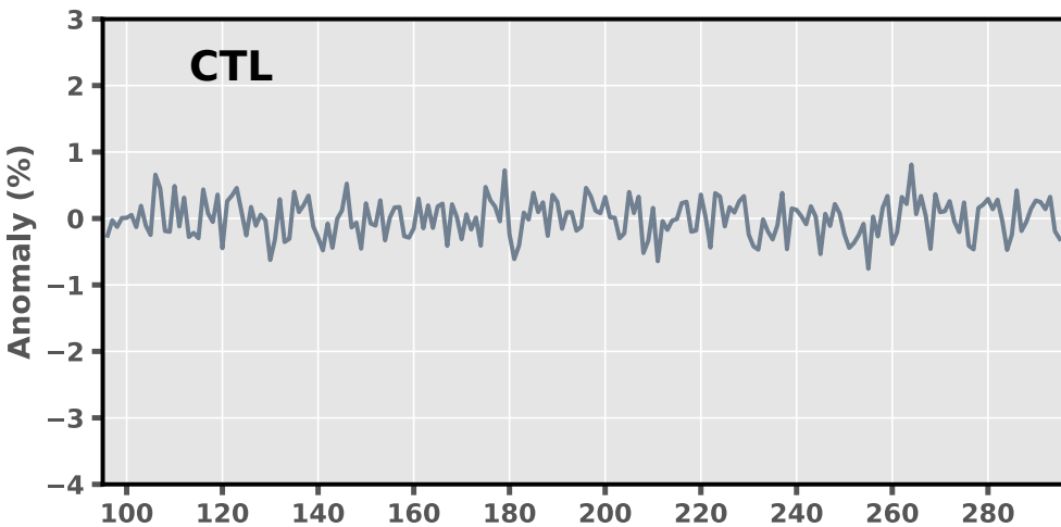
(a) Upper stratosphere
