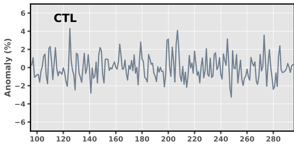
(b) Lower stratosphere
