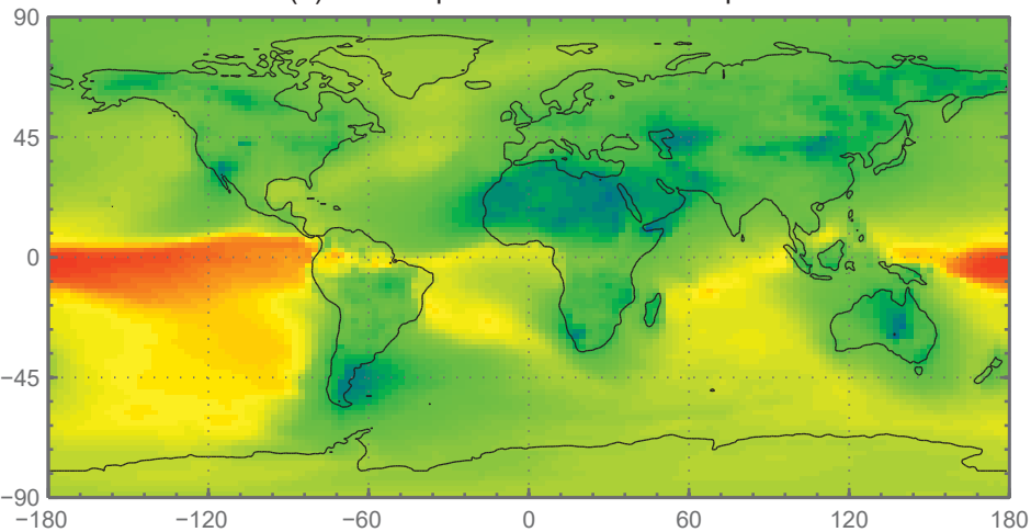
(b) Model percent labile iron < 1 \mu\text{m}
