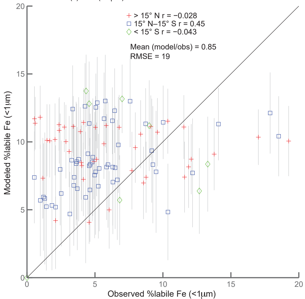
(c) Fine (<1 \mu\text{m} ) %labile FE obs. vs. model r = 0.062
