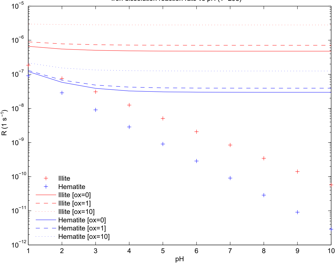
Iron dissolution reaction rate vs pH (T=298)
