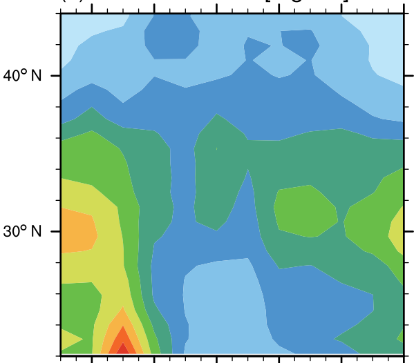
(c) AR5 BC burden [ \text{mg m}^{-2} ]
