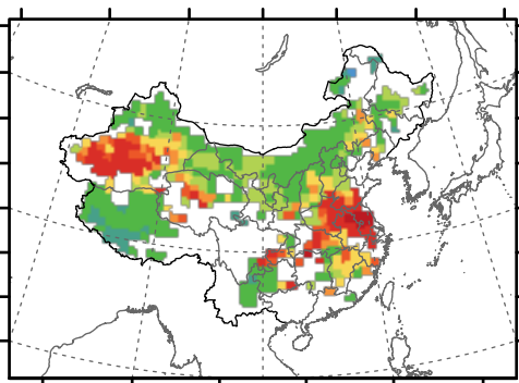
(f) MISR AOD x 2/3
