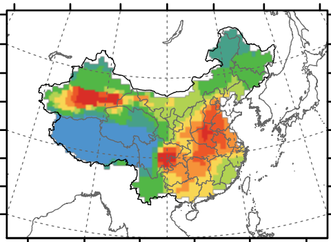
(c) MODIS AOD
