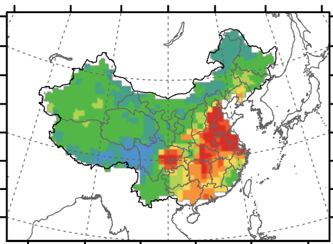
(e) MODIS AOD x 1/2
