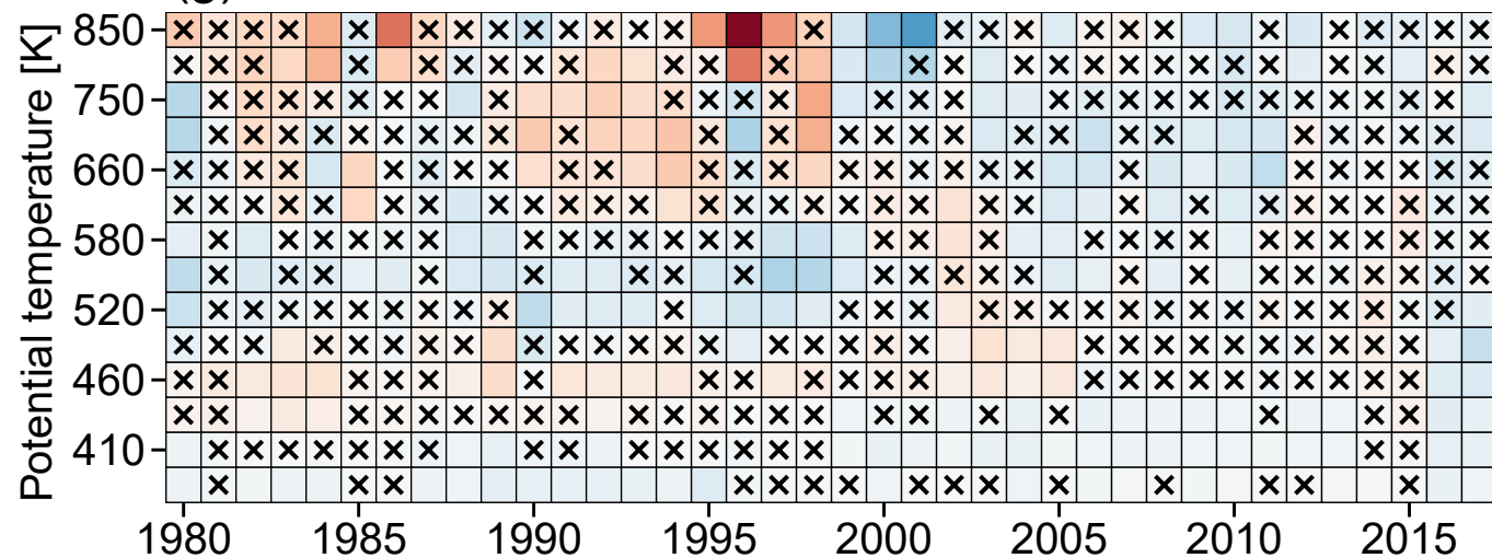
(g) MERRA-2 mean diffs
