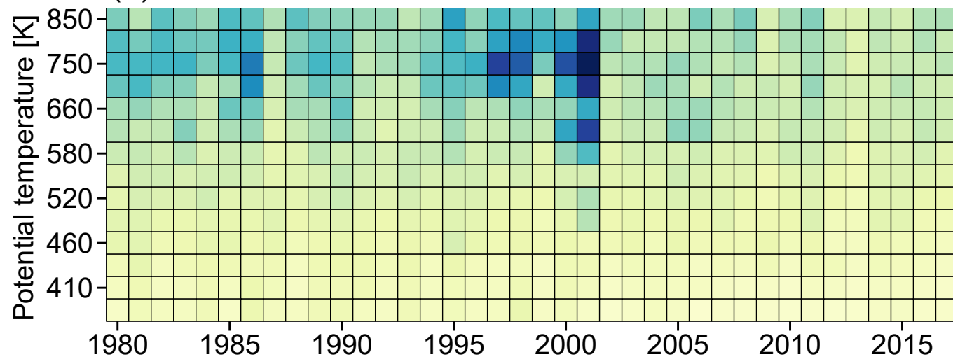
(f) JRA55 SD of diffs
