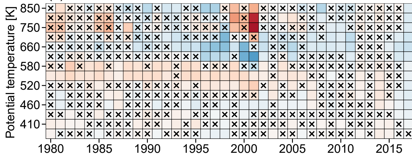
(e) JRA55 mean diffs
