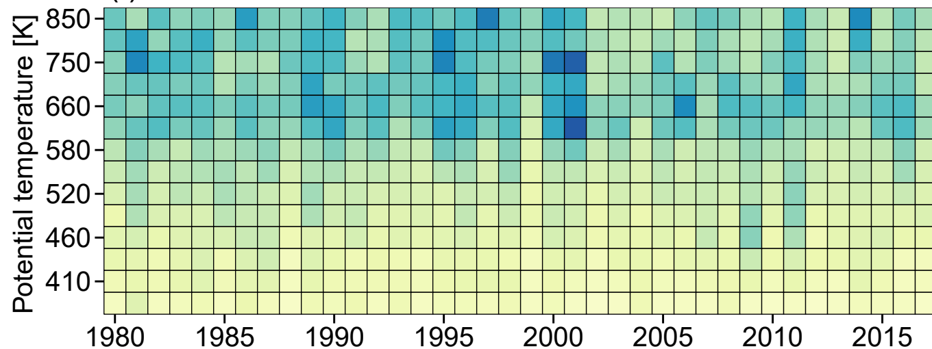
(h) MERRA-2 SD of diffs
