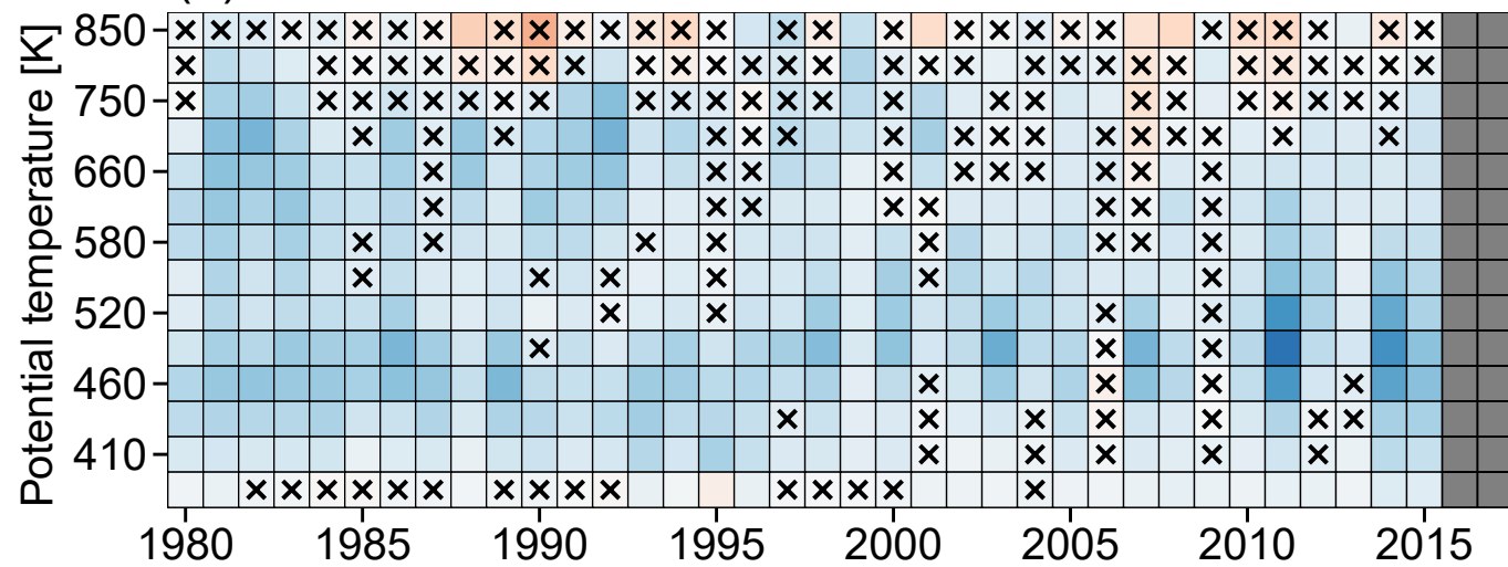
(c) ERA-I mean diffs
