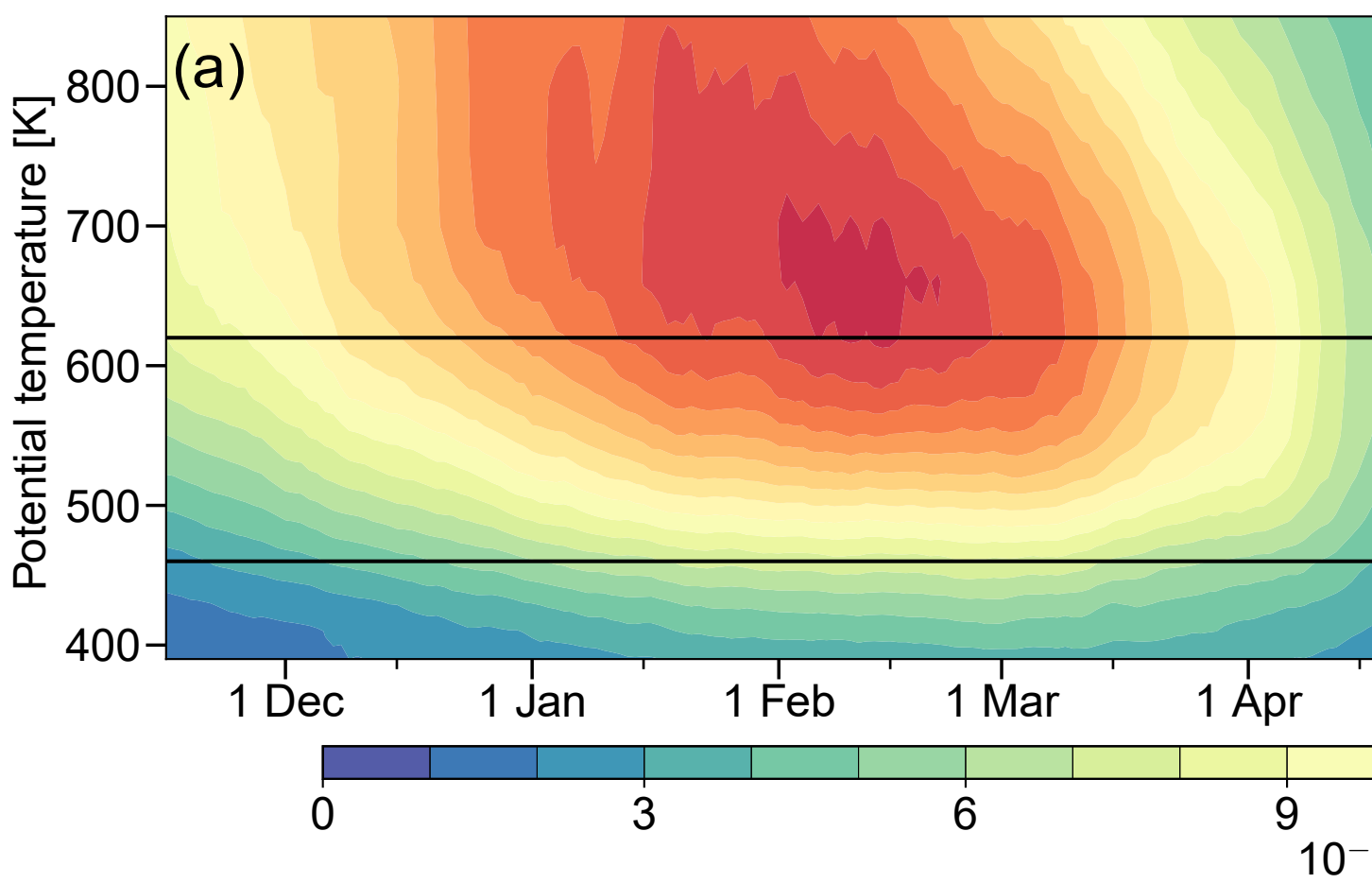
Full climatology (NH winters from 1979/80–2016/17)
