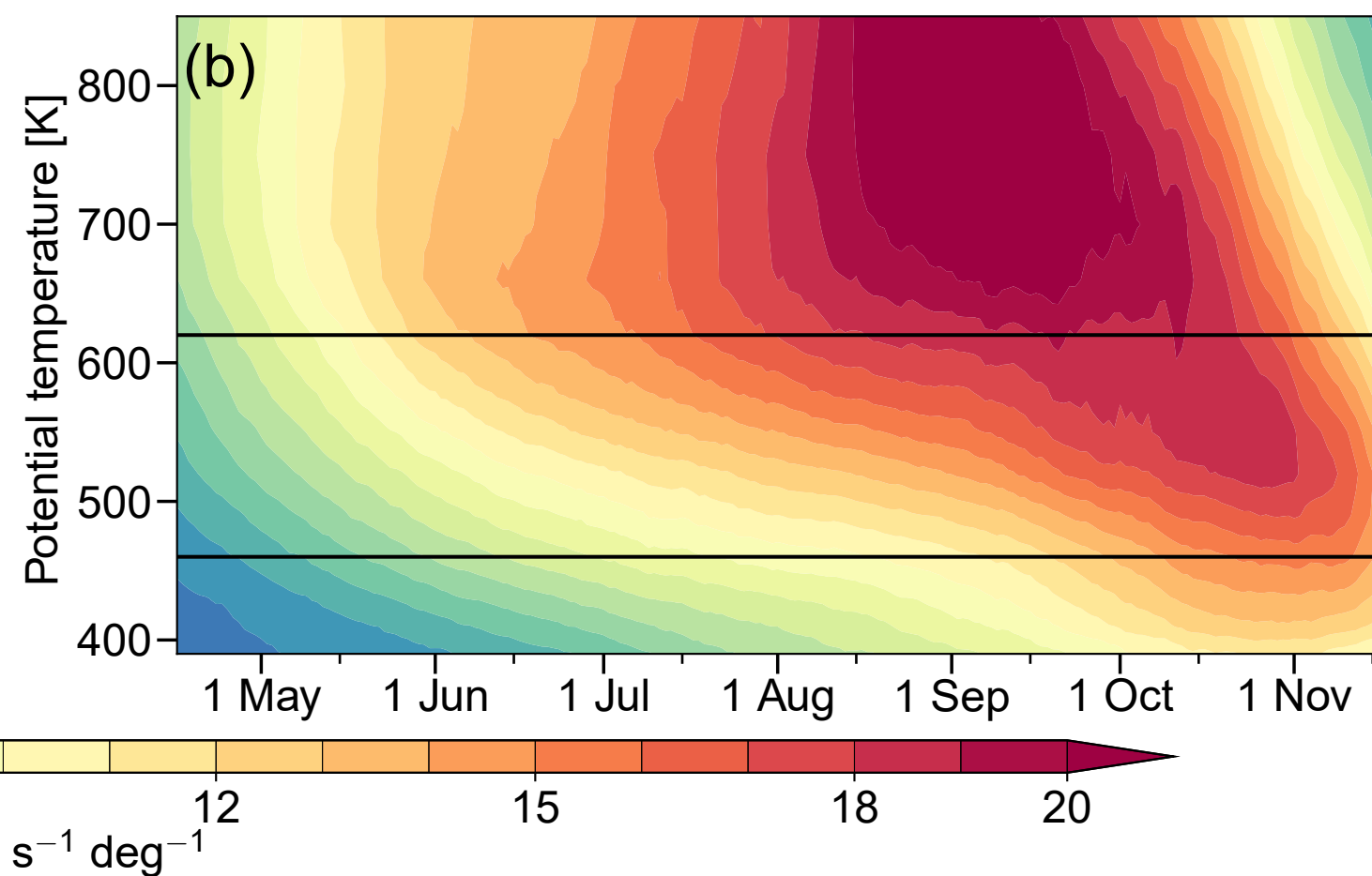
Full climatology (SH winters from 1979–2016)
