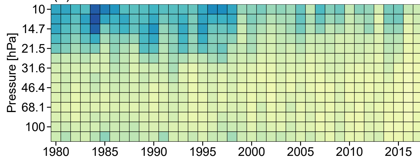
(h) MERRA-2 SD of diffs
