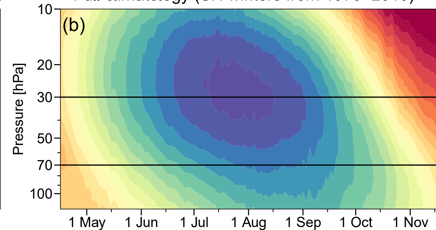
Full climatology (SH winters from 1979–2016)
