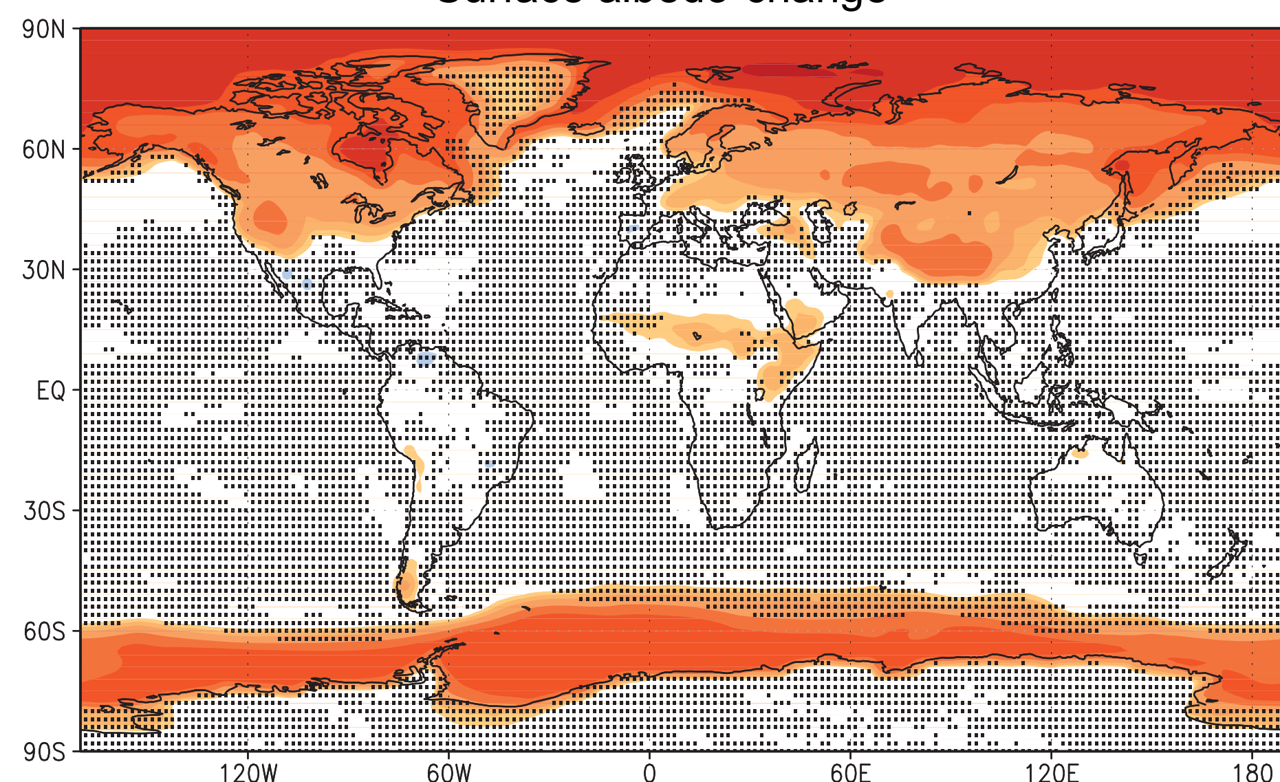
Surface albedo change
