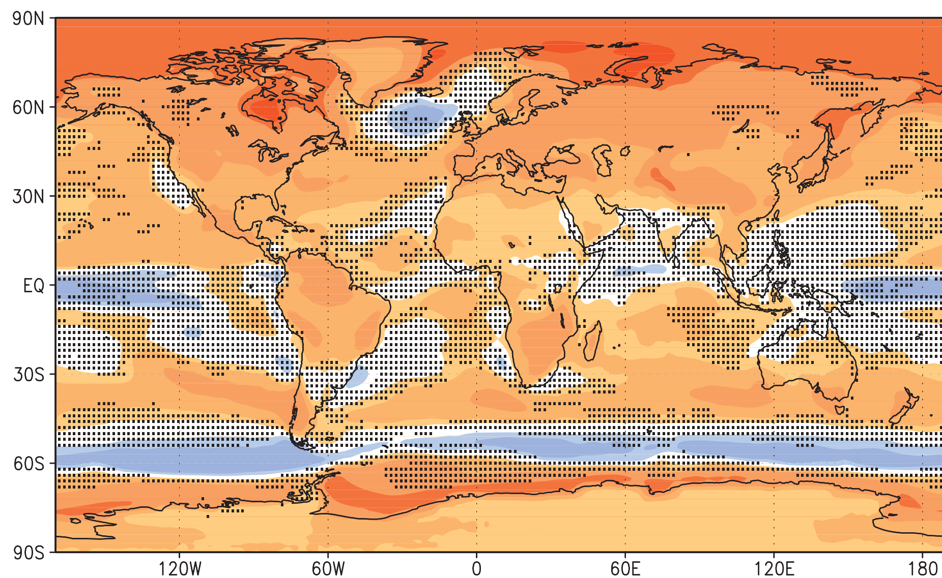
Top of atmosphere albedo change
