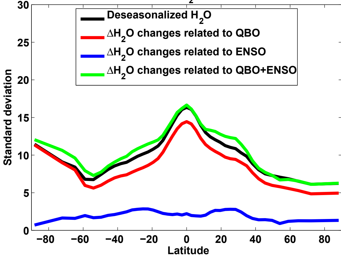
Fraction of variance of the H 2 O anomalies at (380–425 K)
